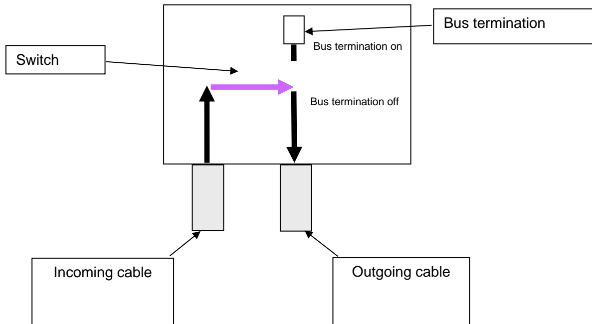
Figure 7: Bus termination off / incoming cable and outgoing cable connected
