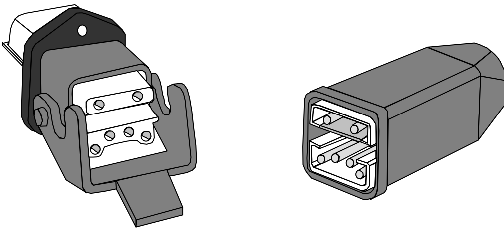
Figure 12: Hybrid connectors
