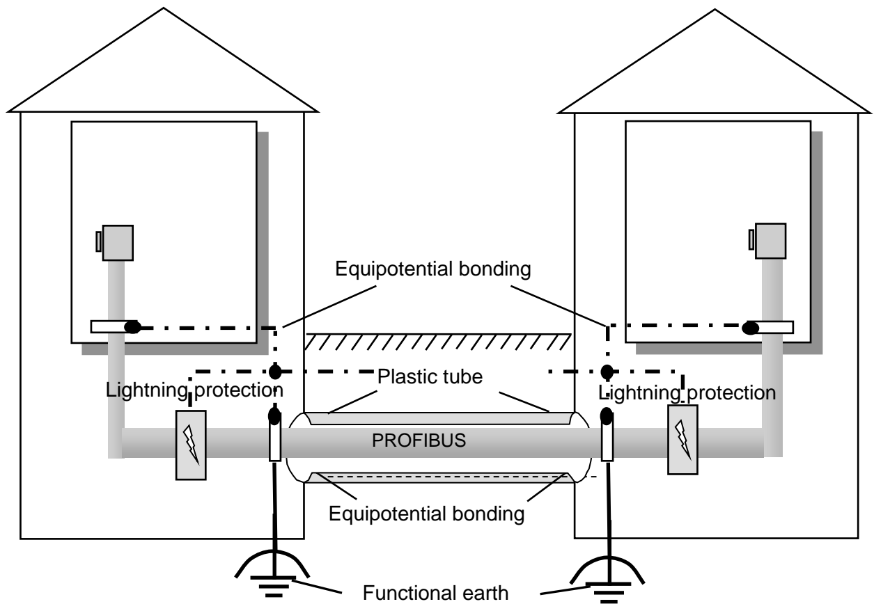
Figure 2: PROFIBUS cables outside of buildings
