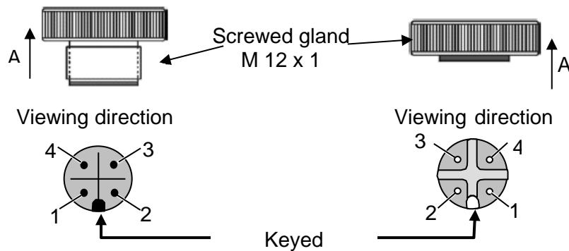
Figure 11: 4-pin M-12 connector (for MBP (PA)) – plug (left) and socket (right)
