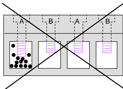
Figure 15: Screw terminals - not suitable for stranded cables without wire-end ferrules
