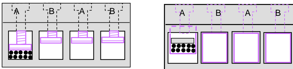
Figure 14: Screw terminals - suitable for stranded cables without wire-end ferrules
