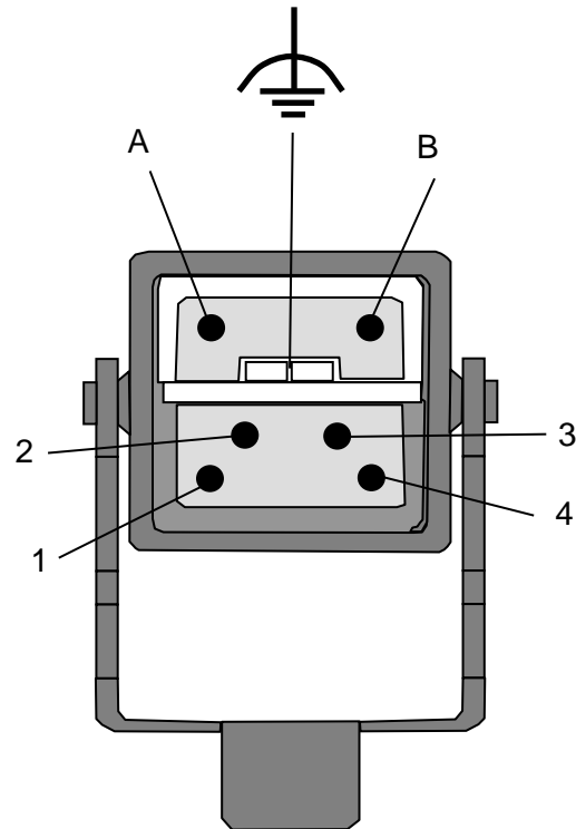
Figure 13: Pin assignment for Hybrid connector by Desina
