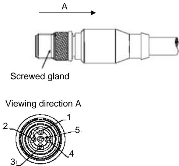
Figure 10: 5 pin M-12 plug for RS 485
