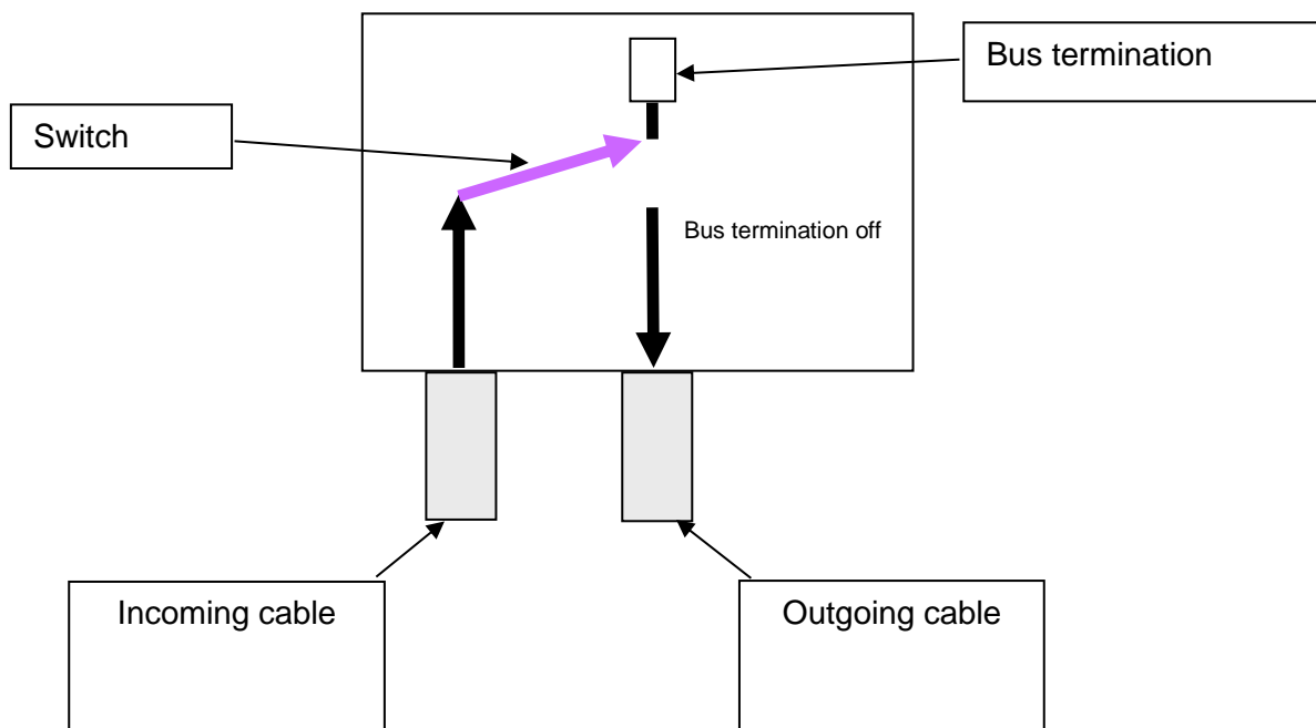
Figure 6: Bus termination on / incoming and outgoing cable not connected
