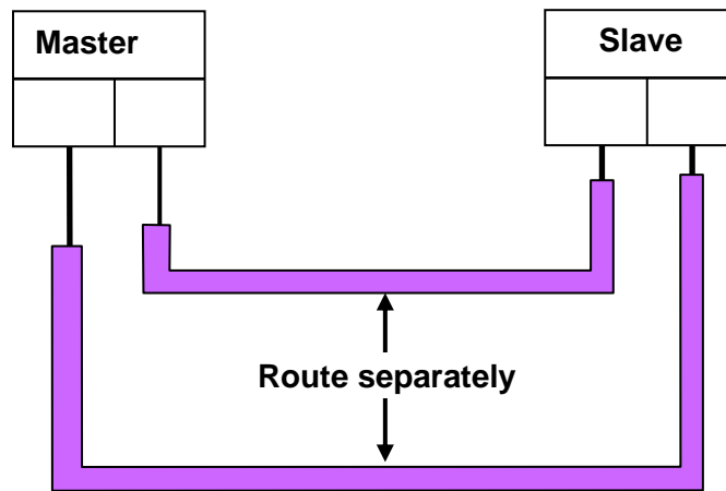
Figure 3: Routing redundant PROFIBUS cables
